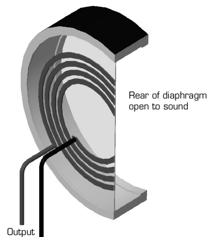
Pressure-gradient transducer – two port
