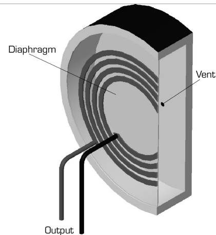
Pressure transducer – single port
